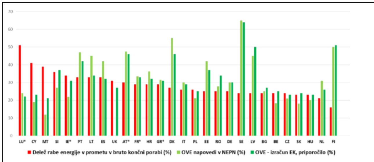
Figure 7: Comparison of projected national RES shares, EC calculations and shares of energy use in transport, source: MzI based on IJS-CEU calculations, 2019
