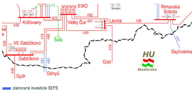
Figure 4: Schematic view of the planned investment project for the construction of new cross-border lines on the SR-HU profile
