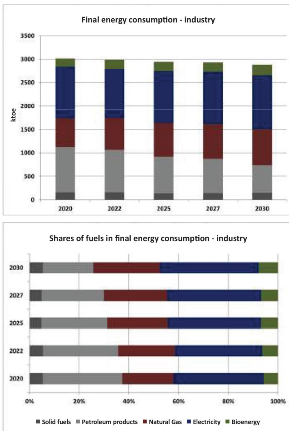
Chart 47: Development of final energy consumption in the industry sector until 2030.
