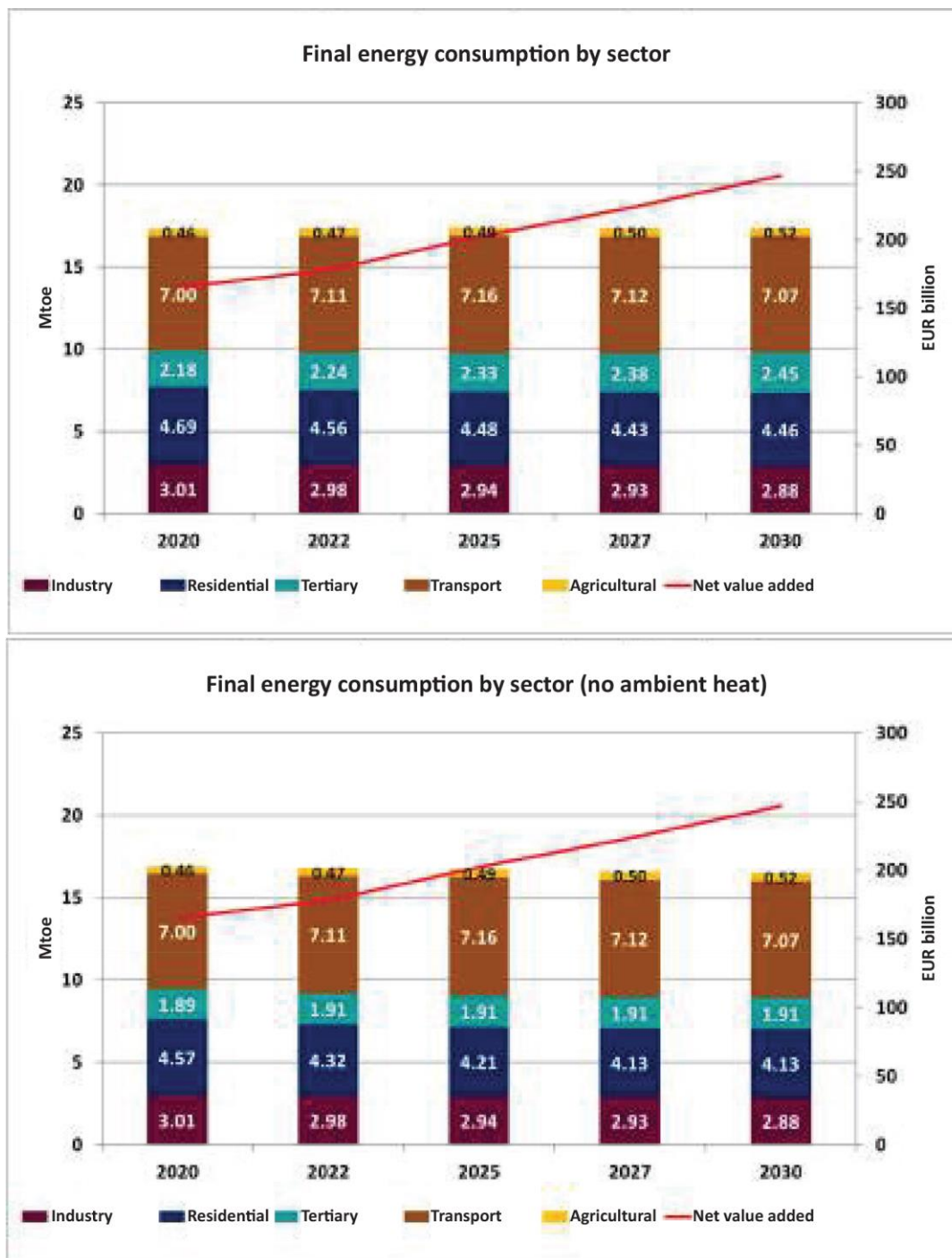
Chart 36: Evolution of final energy consumption by sector by 2030 with and without ambient heat.
