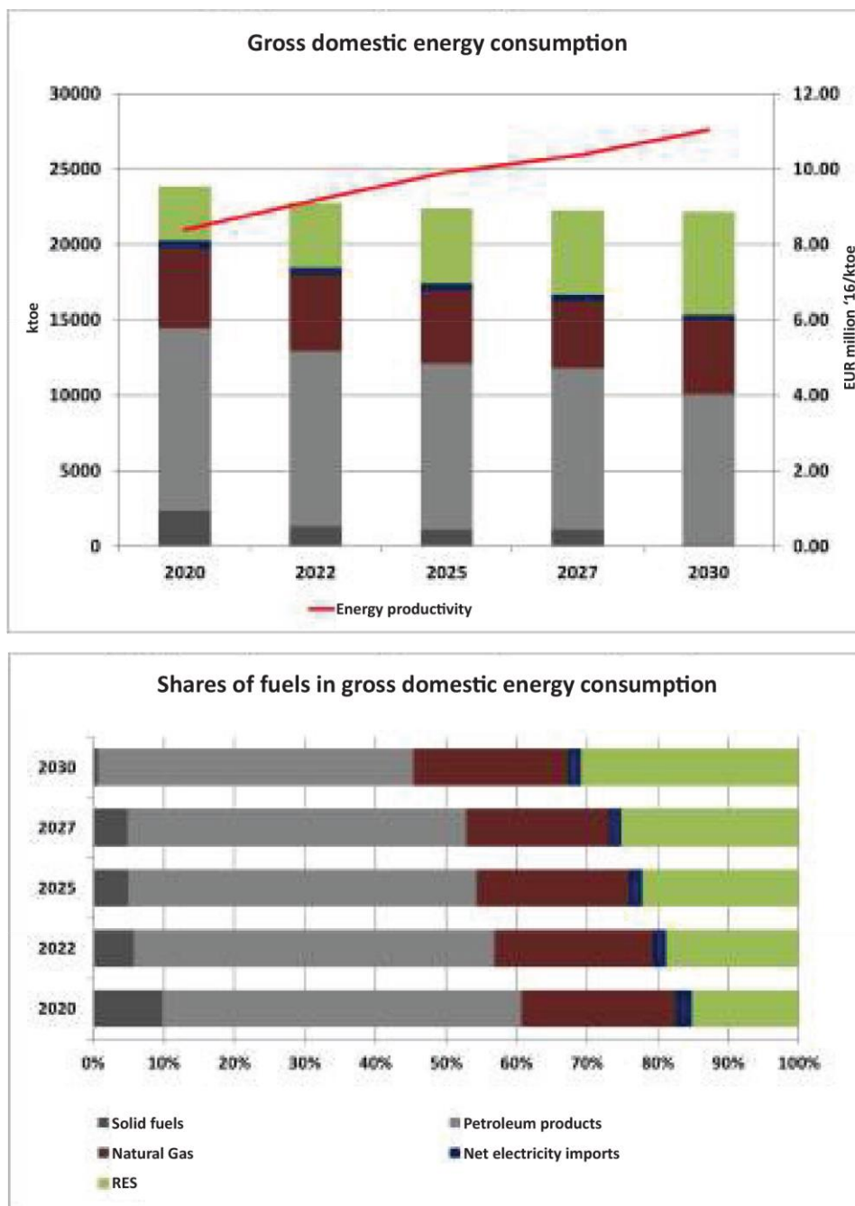
Chart 27: Development of fuels shares in the gross domestic consumption until 2030 for the objectives achievement scenario.
