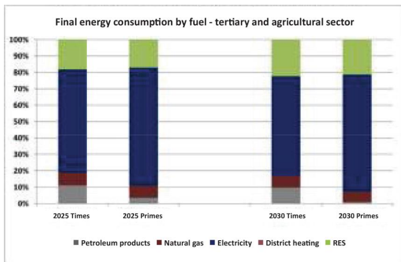
Chart 57: Share of fuel per end sector for the different energy simulations (TIMES – PRIMES).
