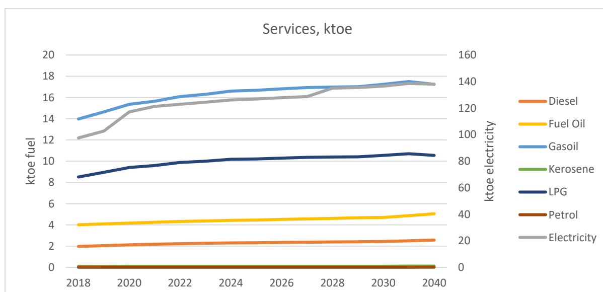
Figure 93 - Final energy consumption split by fuel for services sector under WPM scenario, ktoe
