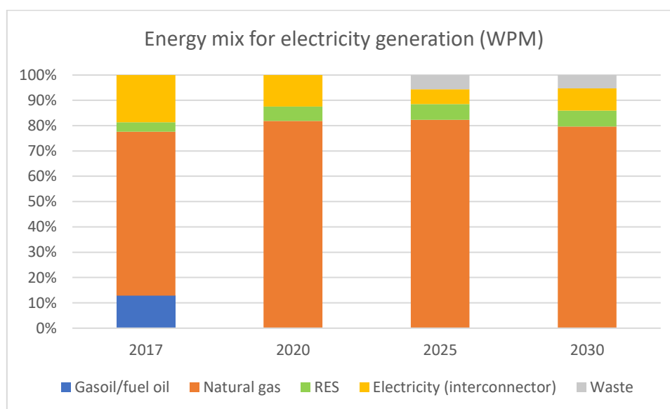
Figure 97 - Energy mix for electricity generation under WPM scenario (%)
