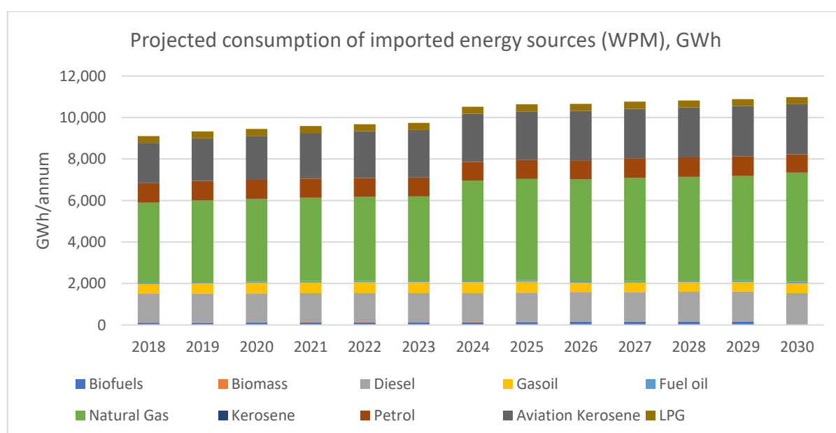
Figure 100 - Projected consumption of imported energy sources (WPM), GWh
