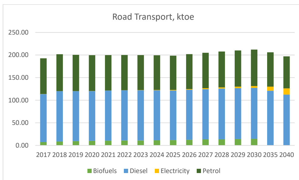
Figure 89 - Projections for final energy consumption for road transport sector, split by fuel, under the WPM scenario, ktoe
