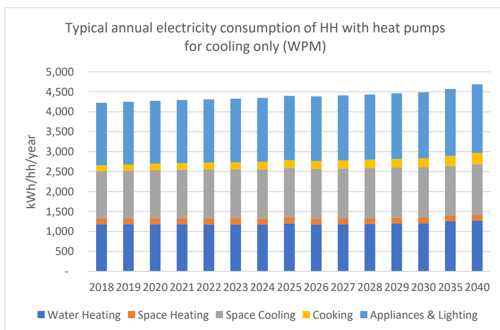
Figure 112 - Typical annual electricity consumption of households with heat pumps for cooling only under WPM (kWh/yr)
