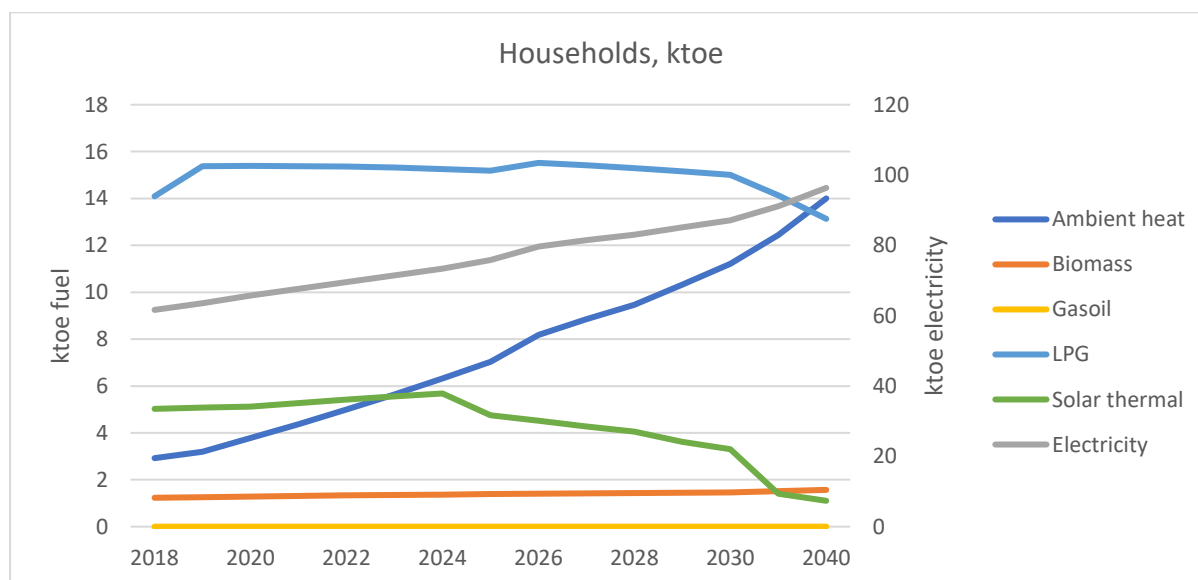
Figure 95 - Final energy consumption split by fuel in residential sector under WPM scenario, ktoe
