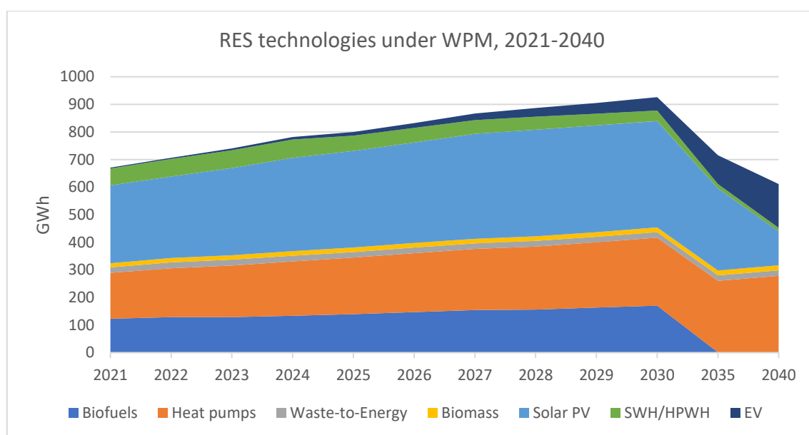
Figure 86 - RES technology consumption under WPM in 2021-2040, GWh
