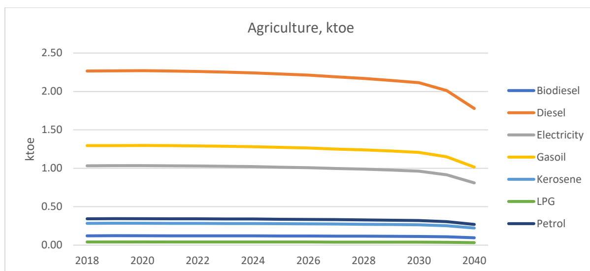
Figure 94 - Final energy consumption split by fuel for agriculture sector under WPM scenario, ktoe
