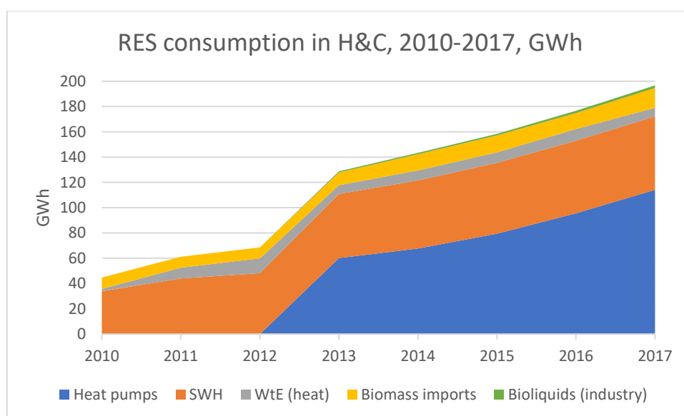
Figure 66 - Renewable energy consumption in H&C, 2010-2017, GWh
