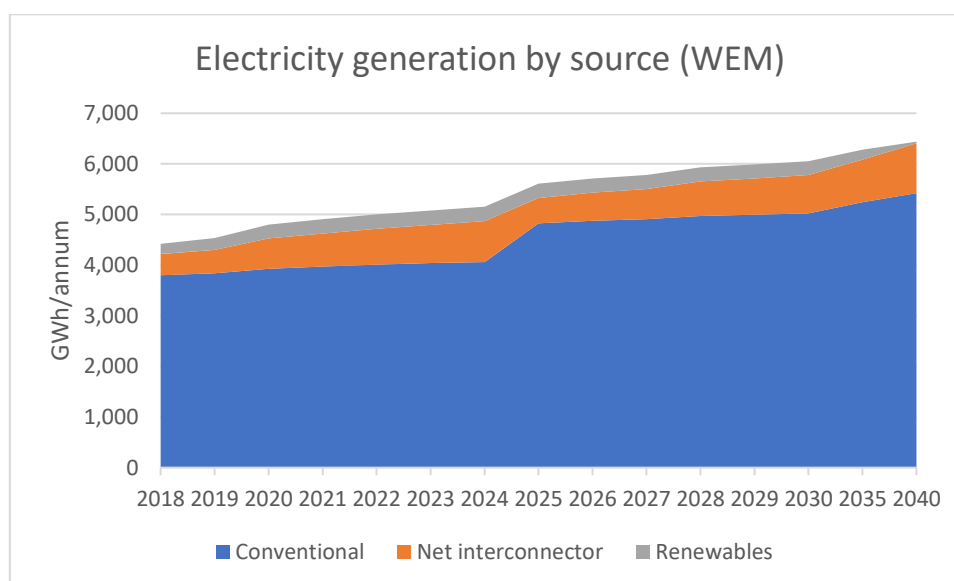
Figure 75 - Electricity generation by source under the WEM scenario, 2018-2040
