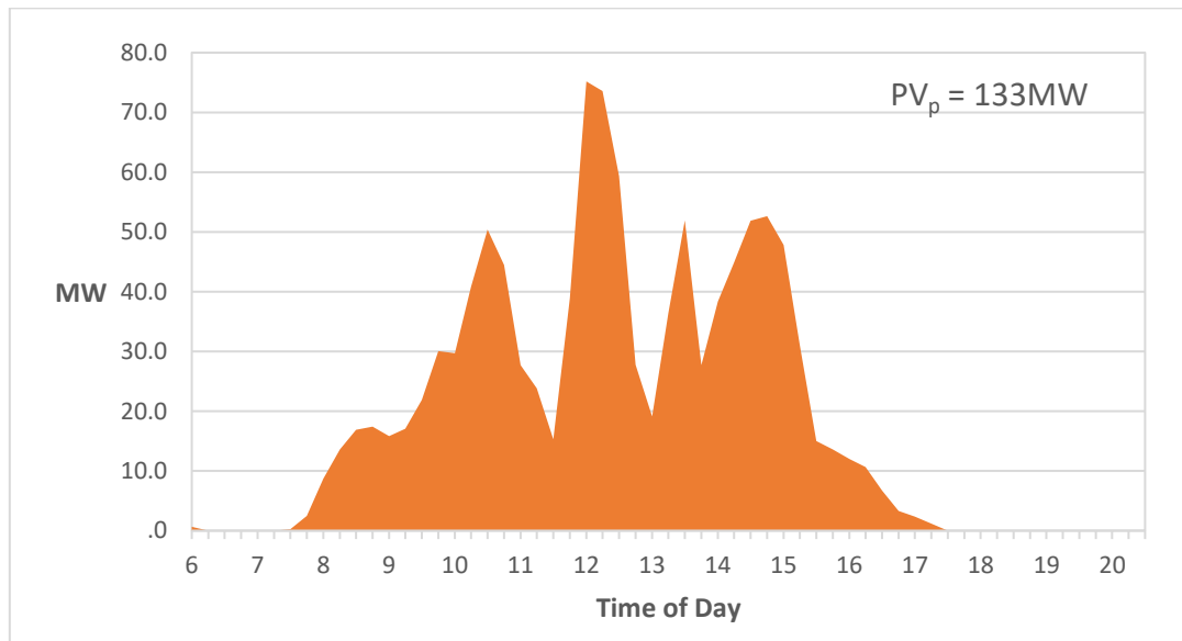
Figure 6 - The effect of cloud cover on electricity generation by 133 MWp of installed solar PV. Transients of circa 60MW are experienced within 60 minutes with the current level of installed capacity
