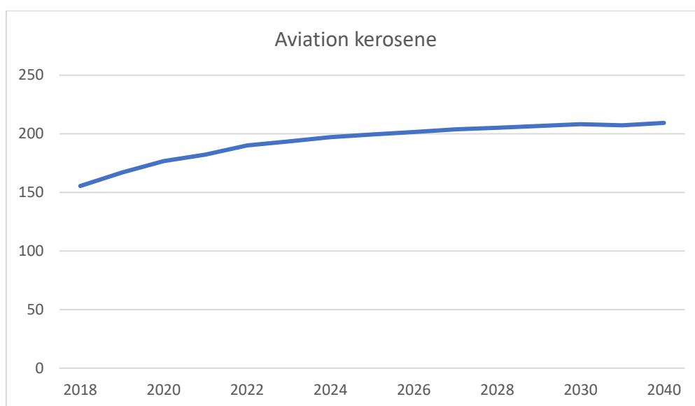
Figure 90 - Final energy consumption in aviation sector under WPM scenario, ktoe
