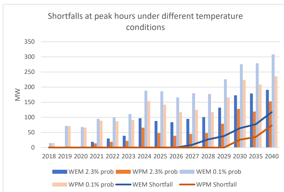
Figure 107 - Shortfalls (MW) at peak hours under different temperature conditions: (i) normal climate; (ii) extreme temperature with a 2.3% probability; and (iii) extreme temperature with a 0.1% probability.
