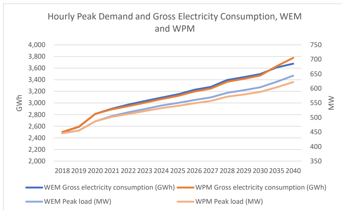
Figure 103 - Peak load (MW) and gross electricity consumption (GWh) under WPM and WEM scenario, 2018-2040
