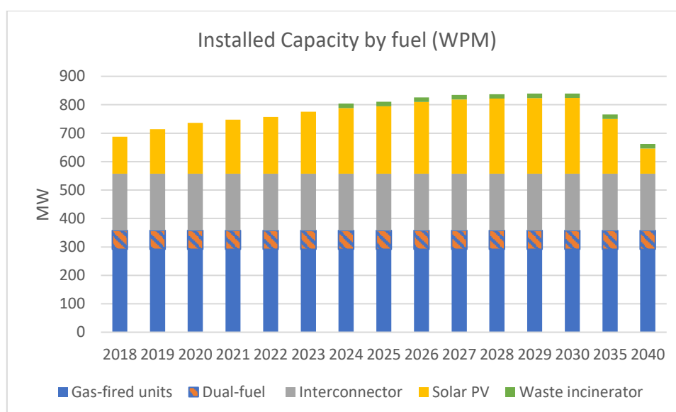
Figure 102 - Installed capacity by source under WPM scenario (MW), 2018-2040
