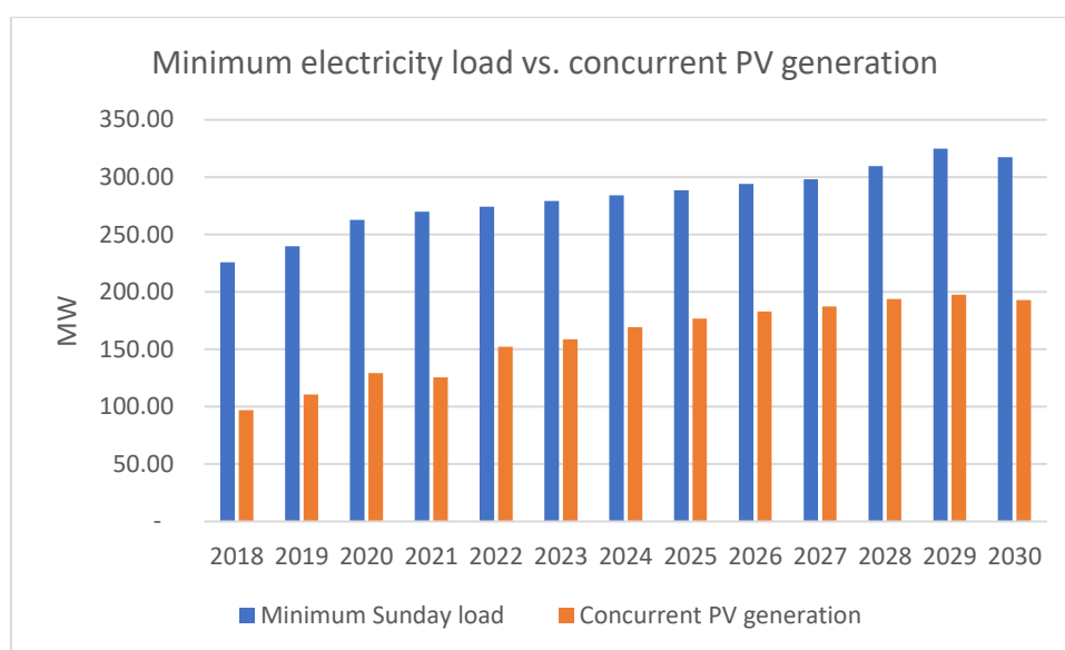
Figure 108 - Projected minimum Sunday load and concurrent PV generation under WPM scenario (MW)
