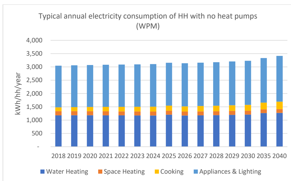
Figure 113 - Typical annual electricity consumption of households with no heat pumps under WPM (kWh/yr)
