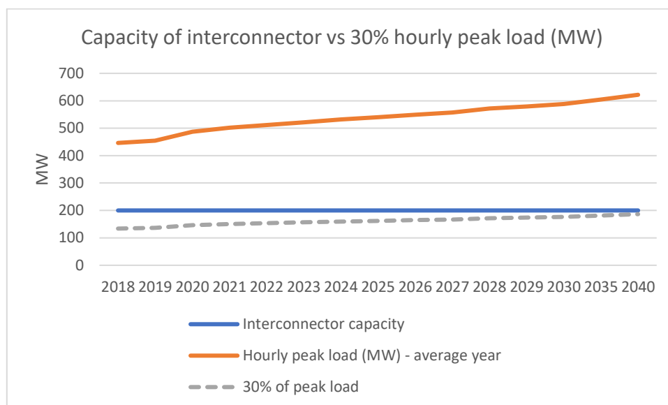
Figure 19 - Nominal transmission capacity of interconnector vs 30% of peak load (WPM), 2018-2040
