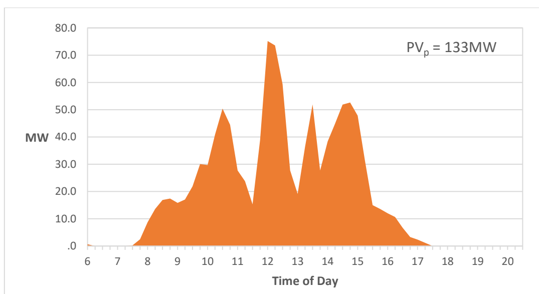
Figure 21 – Solar PV generation during a typical day in April with intermittent cloud cover (MW)
