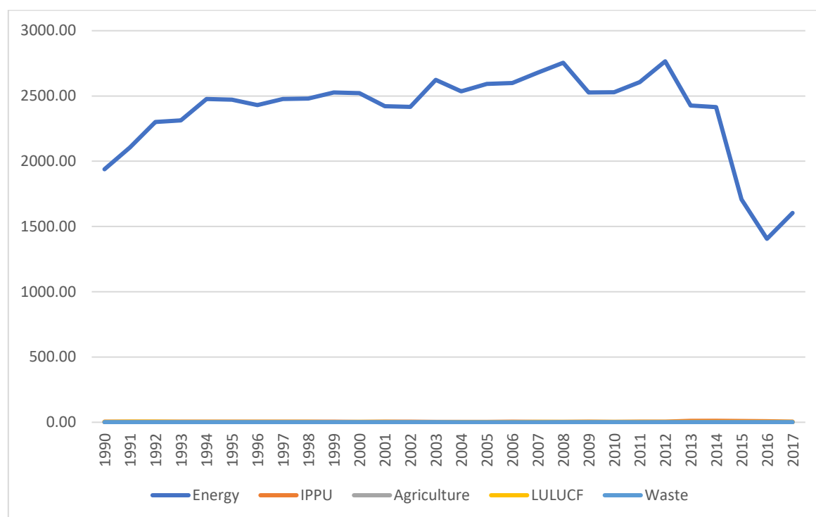
Figure 39 - CO 2 emission trends by sector
