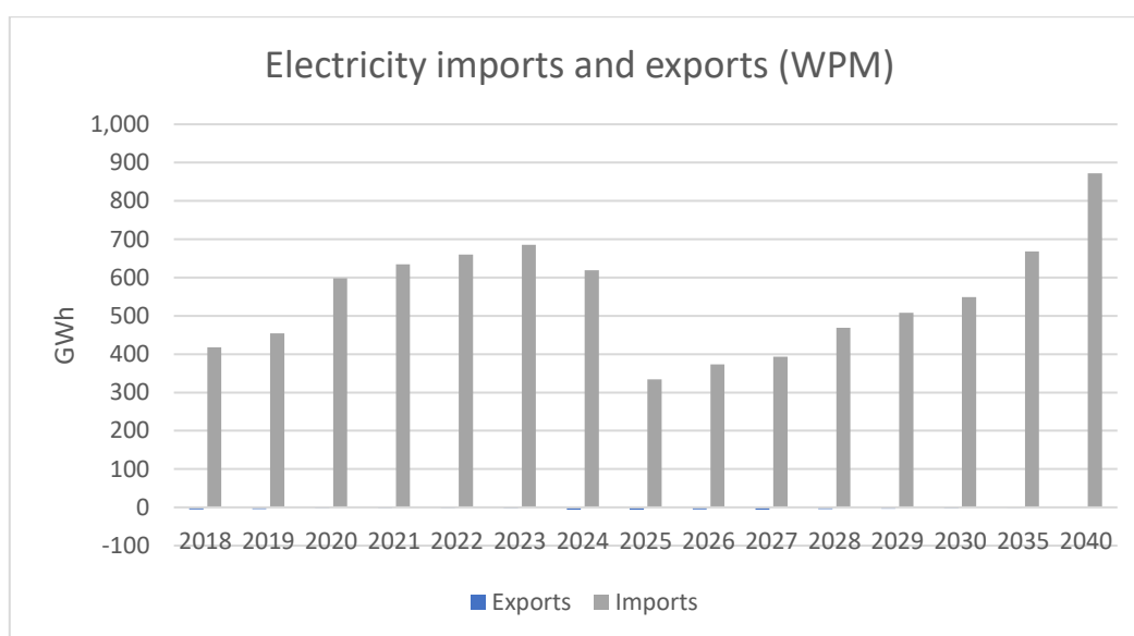
Figure 105 - Electricity imports and exports over the interconnector (WPM), 2018-2040
