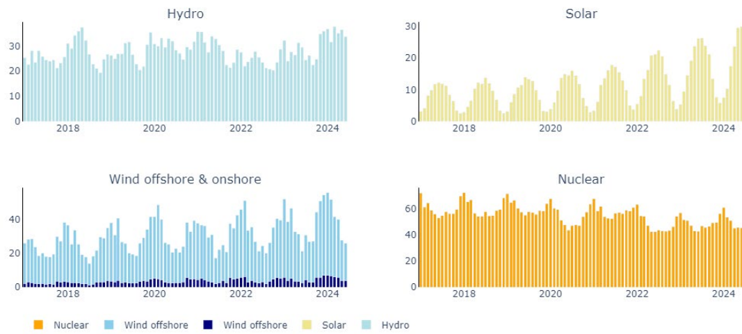
Figure 44 - Monthly renewable and nuclear generation in the EU (TWh)
